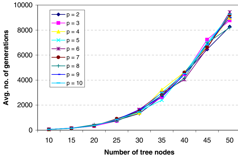
Fig. 2. Average number of generations for trees with fixed number of sons p
